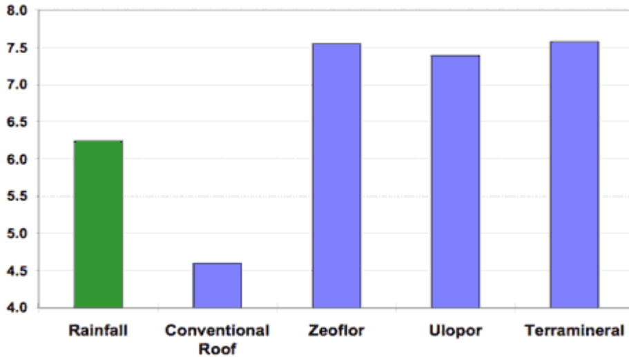
Illustration 5: pH (median) of the runoff from the tested substrates between 8/7/97 and 1/21/98
