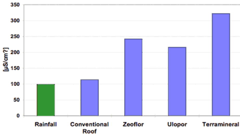
Illustration 3: Electrical conductivity (median) of the runoff from tested substrates between 8/7/97 and 1/21/98.
