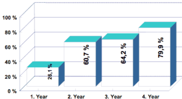
Illustration 2: Development of phosphate retention after installation of green roof (retention as percentage of influx)
