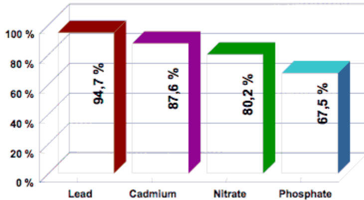
Illustration 1: Retention of contaminants by extensive green roofs (retention as percentage of influx)
