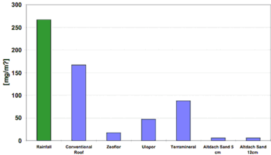
Illustration 8: Total nitrogen discharged from 8/7-11/3/97 and from 1/8 –1/21/98
