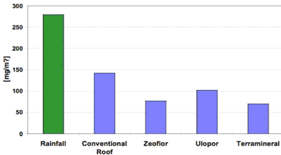
Illustration 10: Discharge of o-PO 4 -P from 8/7-11/3/97 and from 1/8 –1/21/98
